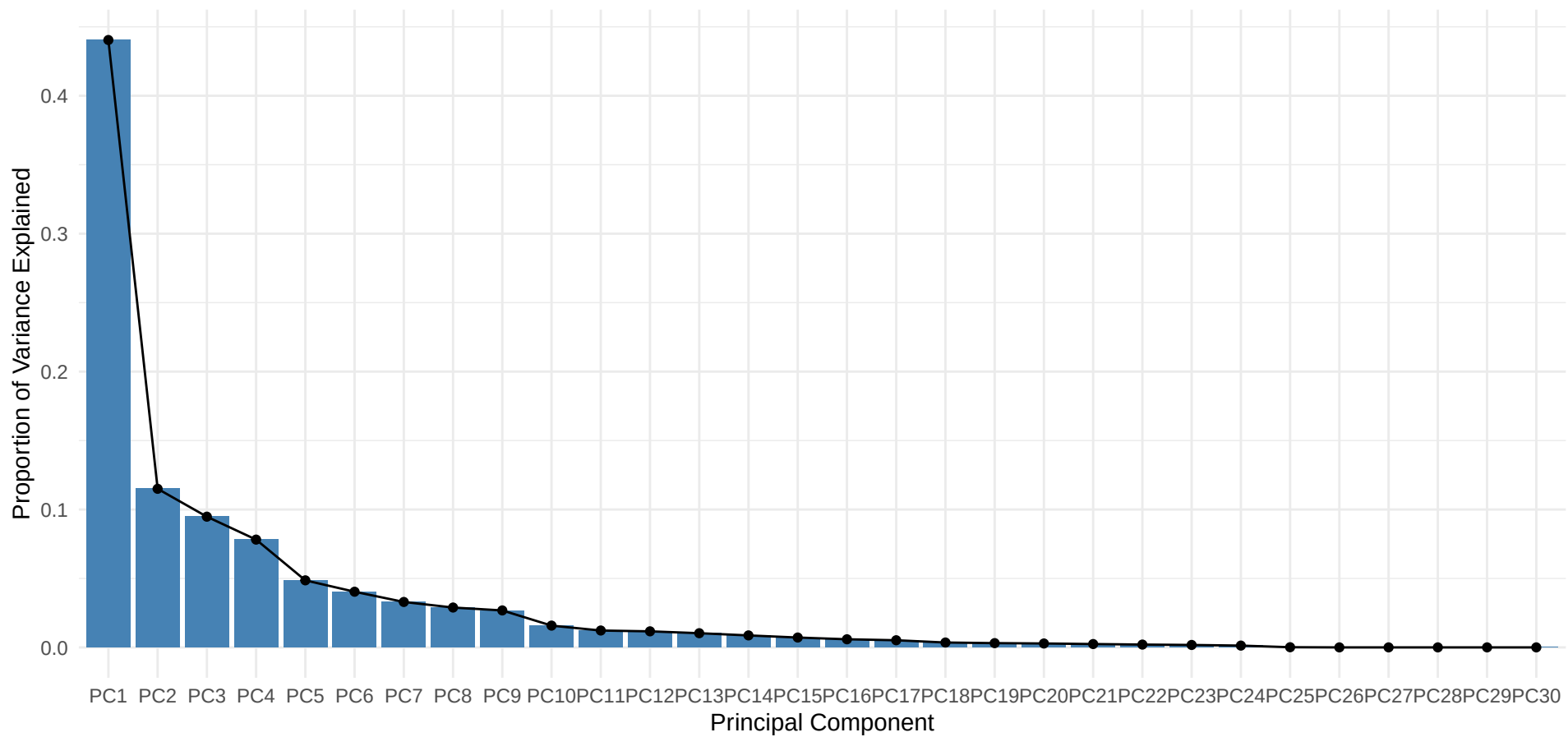
Scree Plot of PCA for FLARE010
